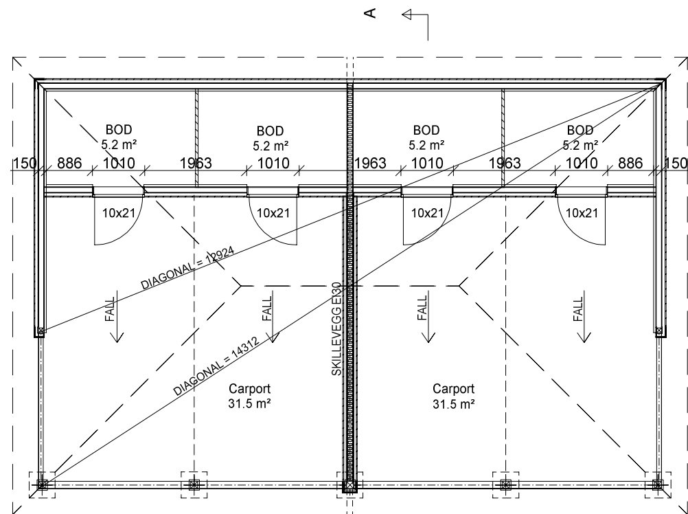
PLAN CARPORT/BOD BYA = 95.6 m 2
